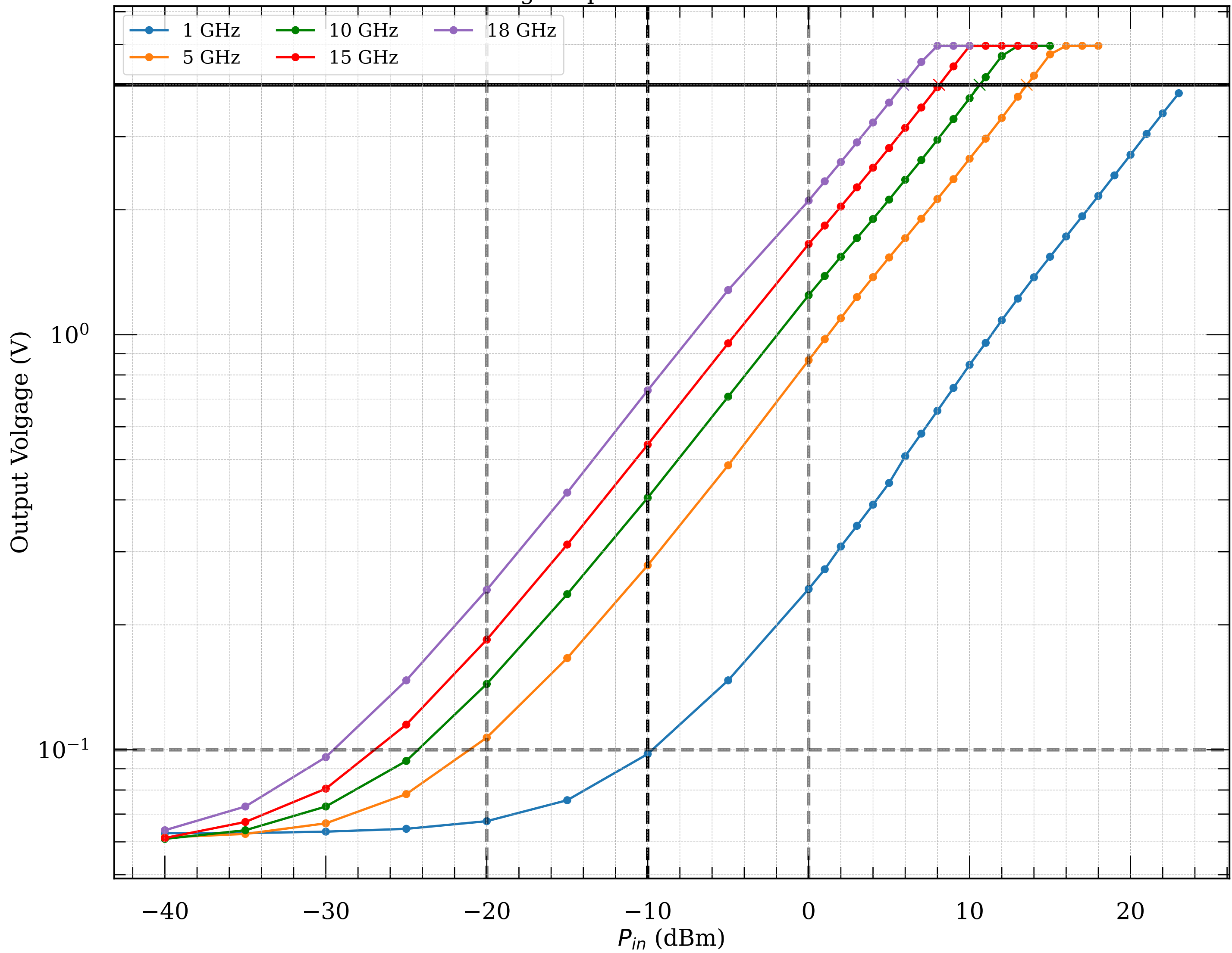
Measured voltage-to-power curve of detector module040
